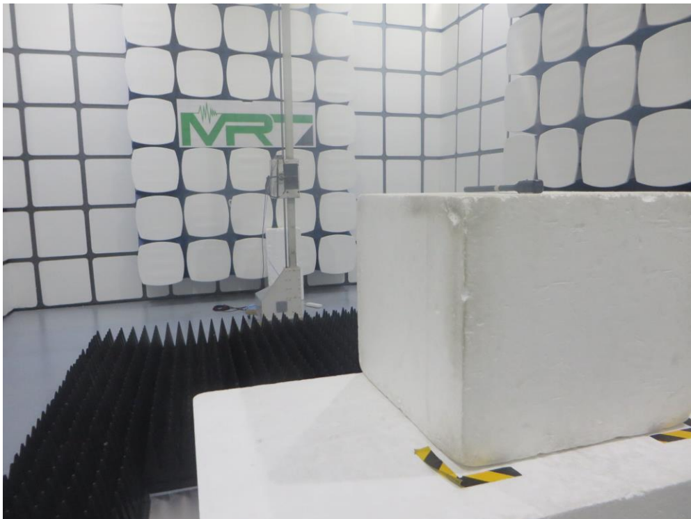
Description: Radiated Emission Test Setup Above 1GHz
