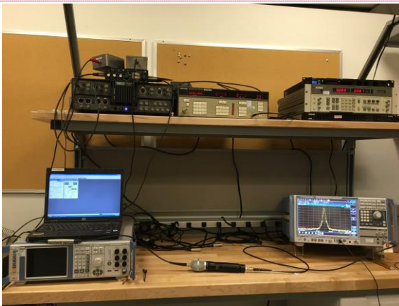
Figure B-1 - Test Setup for Necessary Bandwidth
