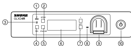
Panel delantero
