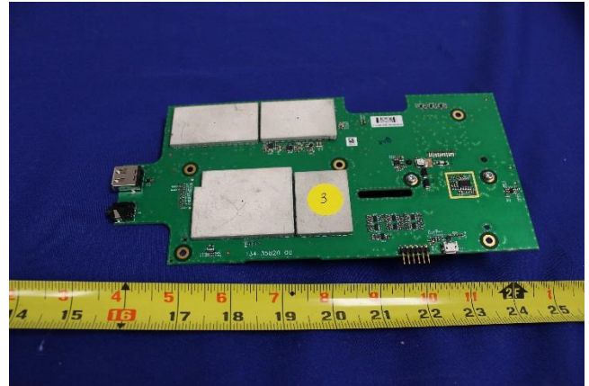
Modem Board-1 Bottom View
