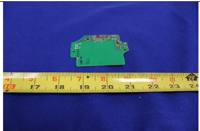
Modem Board-3 Bottom View
