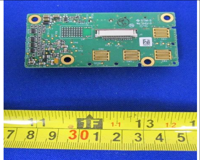
PCB Board 3 Bottom View
