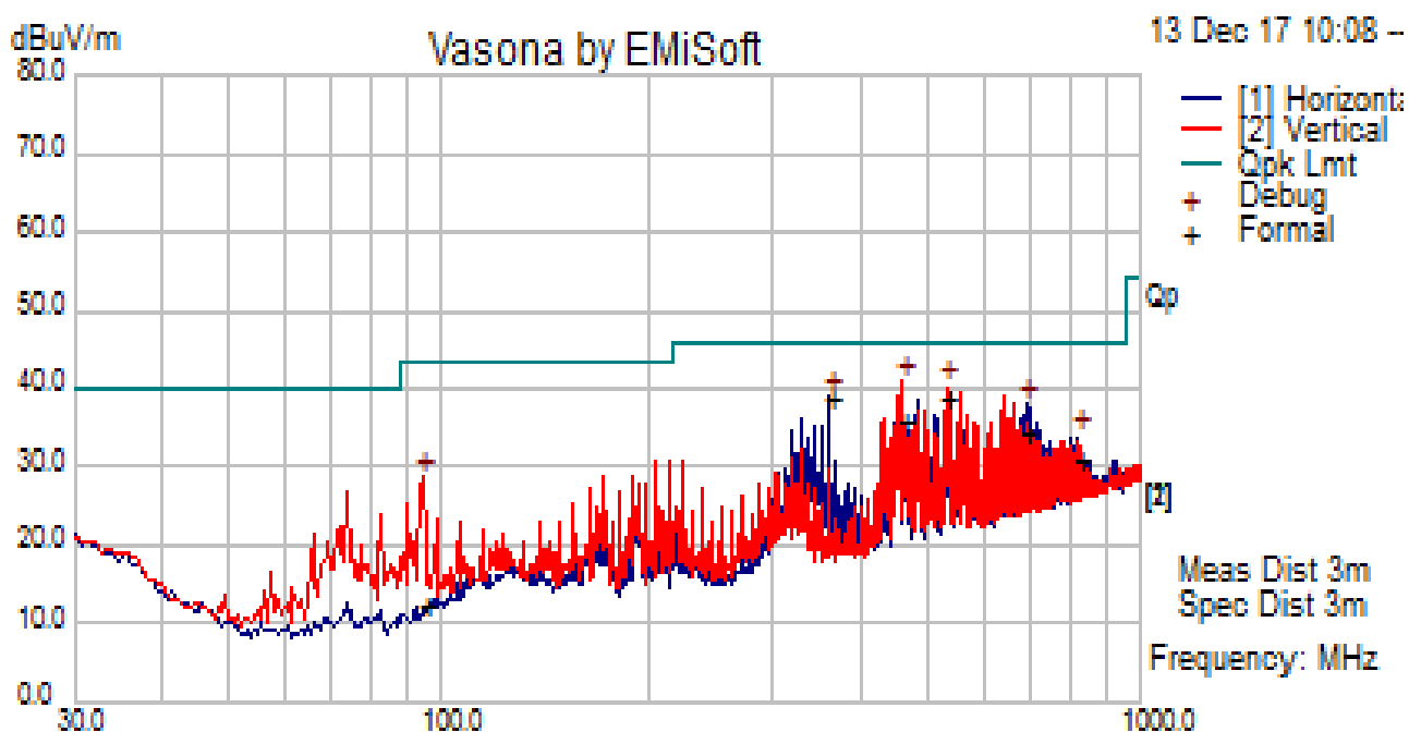
f=30MHz – 1000MHz Measurements
