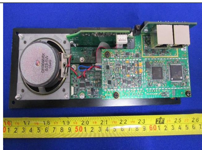
EUT Open Case View 2
