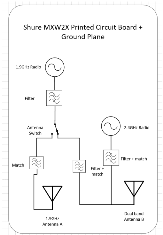
Figure 1-2. Shure MXW2X Antennas Block Diagram
