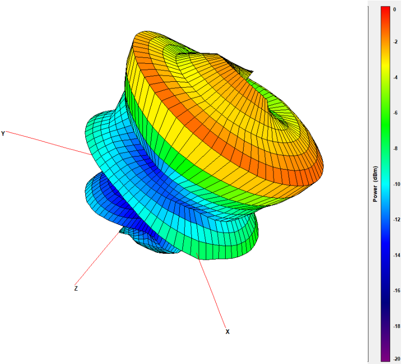
Figure 3-4. 1.9GHz Antenna B 3D
