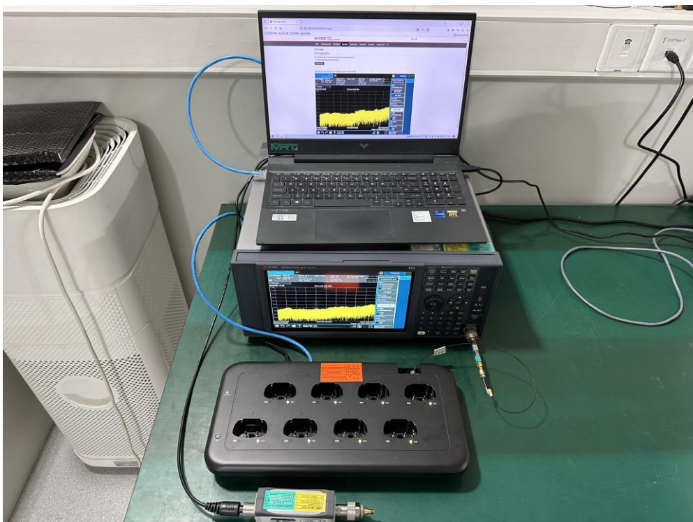
Description: RF Conducted Test Setup – MXWNDX8
