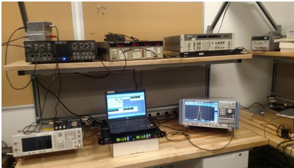
Figure B-1 Test Setup for Necessary Bandwidth
