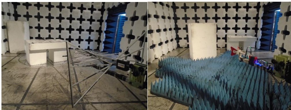
Figure B 1: QLXD1 Transmitter Test Setup
