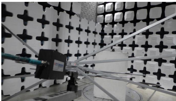
Figure 1: QLXD1 Transmitter Test Setup
