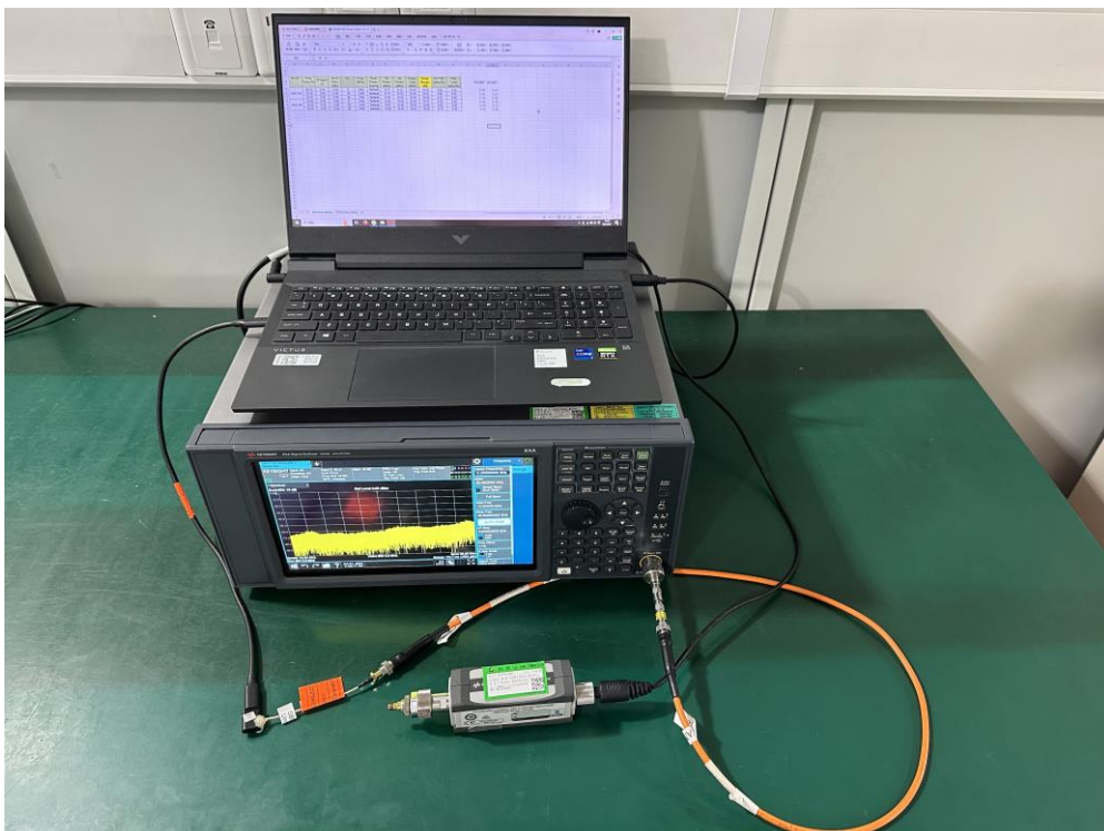
Description: RF Conducted Test Setup for BLE
