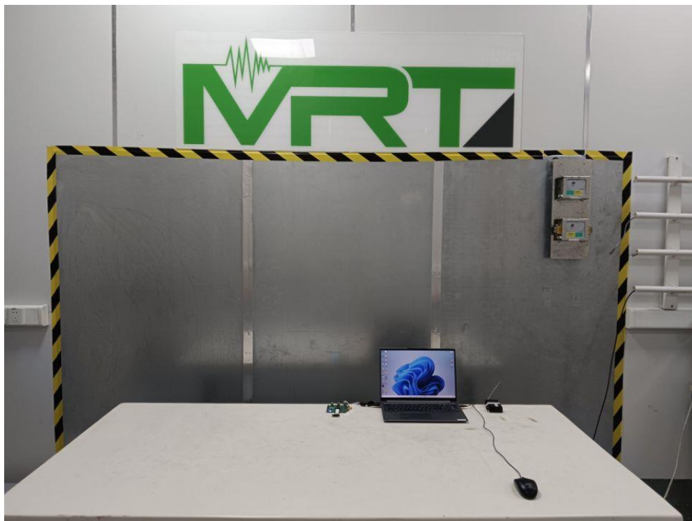
Description: Front View of Conducted Emission Test Setup for Power Port
