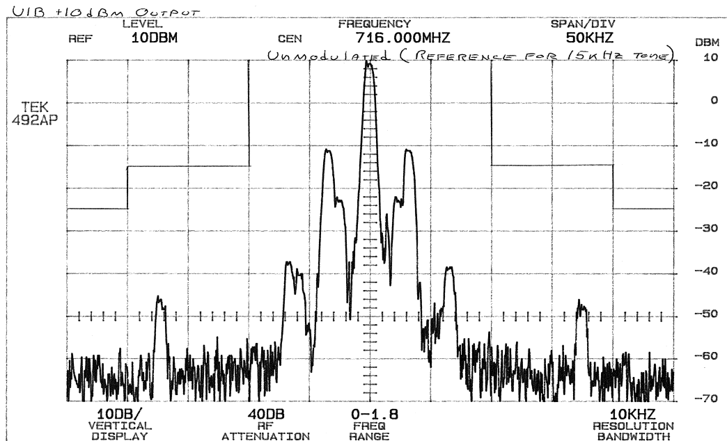
U1B 716 15kHz Reference
