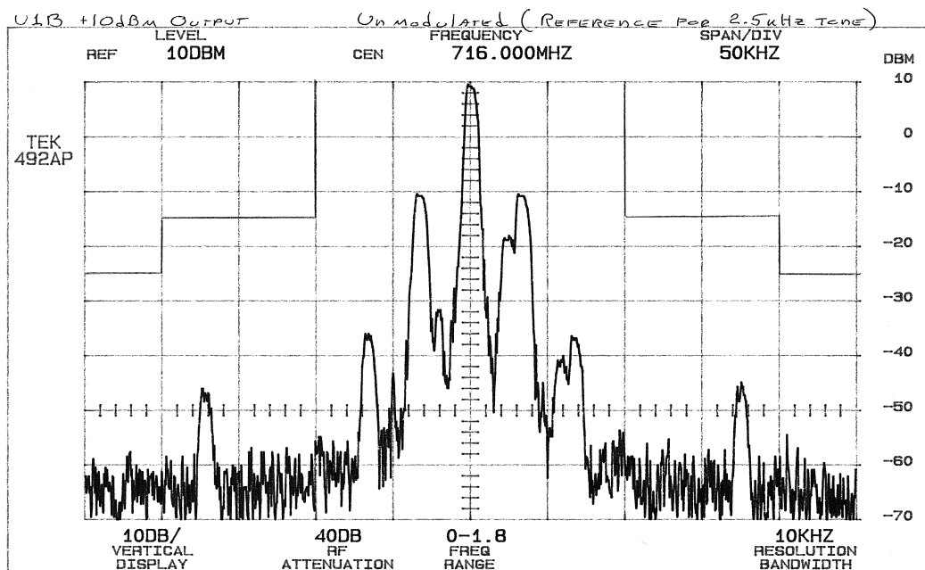
U1B 716 2.5kHz Reference
