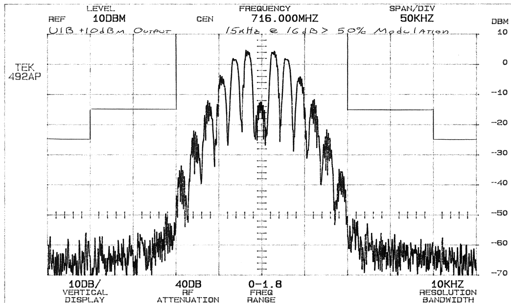
U1B 716 15kHz @+16dB >50% Modulation
