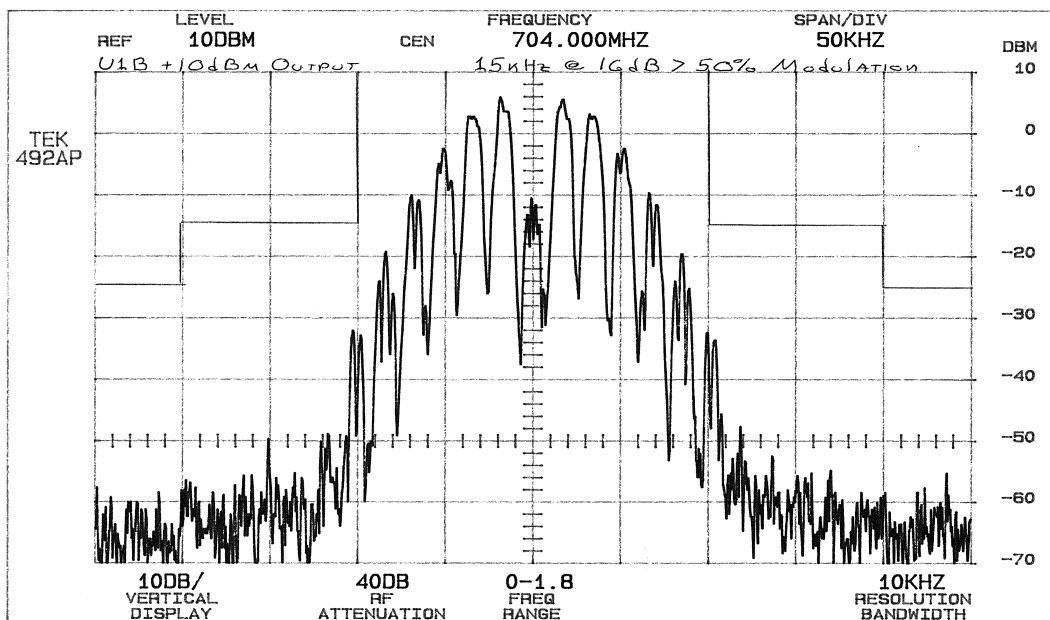
U1B 704 15kHz@+16dB >50% Modulation
