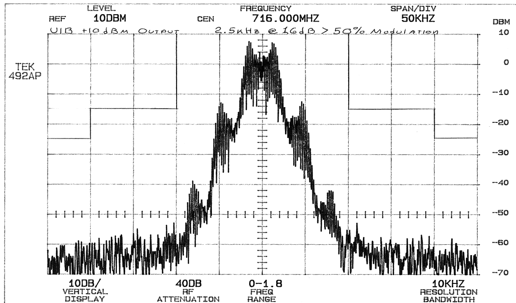
716 2.5kHz U1B @ +16> 50% Modulation
