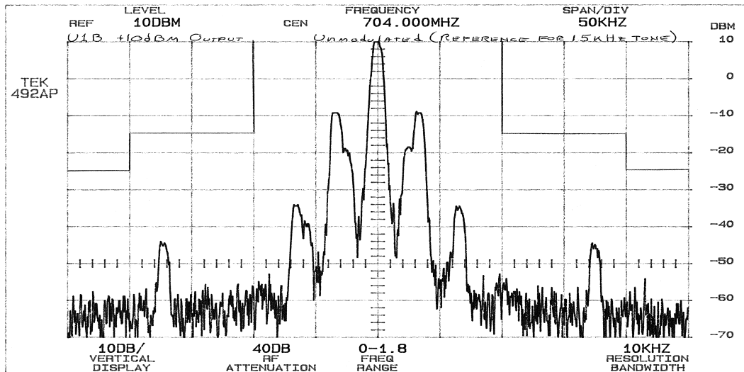
U1B 704 15kHz Reference
