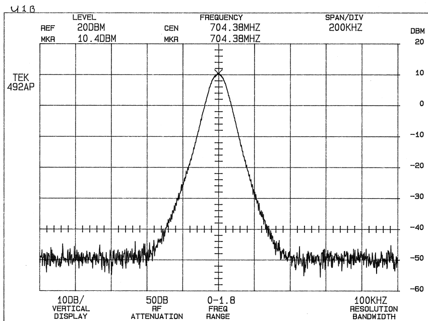
U1B Conducted Output @ 704 mHz
