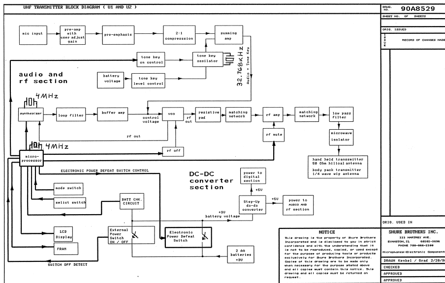
U2B Block Diagram
