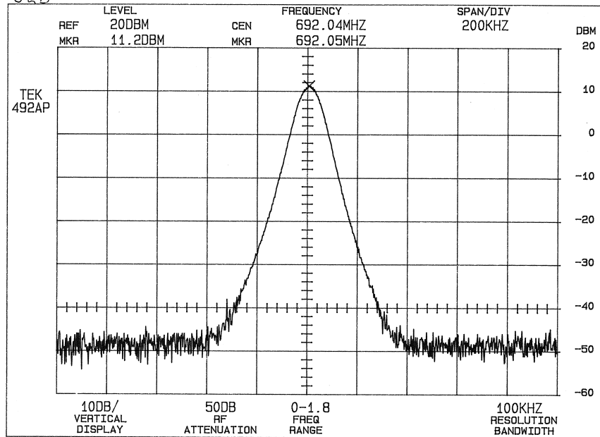
U2B Conducted Output @ 692 mHz
