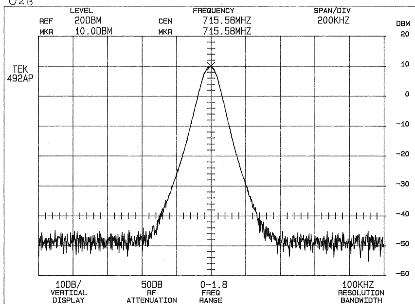
U2B Conducted Output @ 715 mHz
