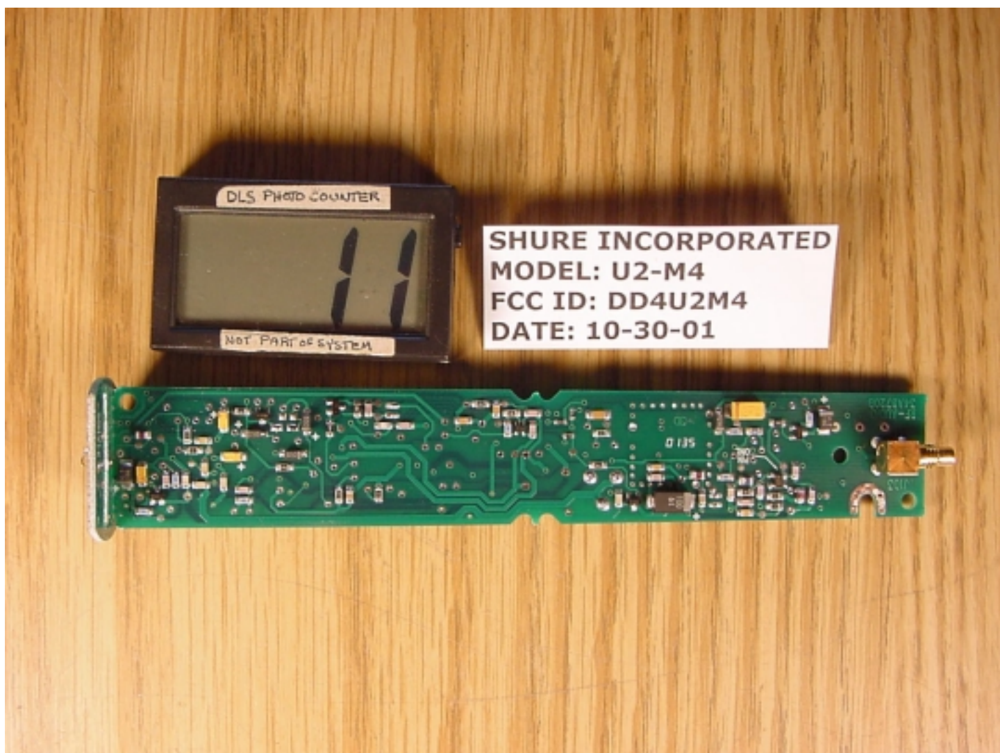
RF – Audio Board Side 2
