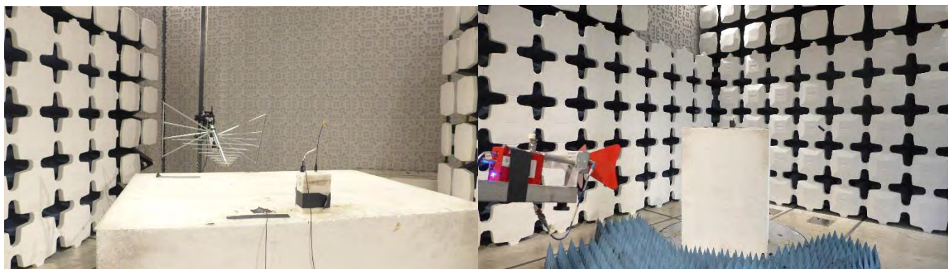
Figure B 1: ULXD1 Transmitter Test Setup
