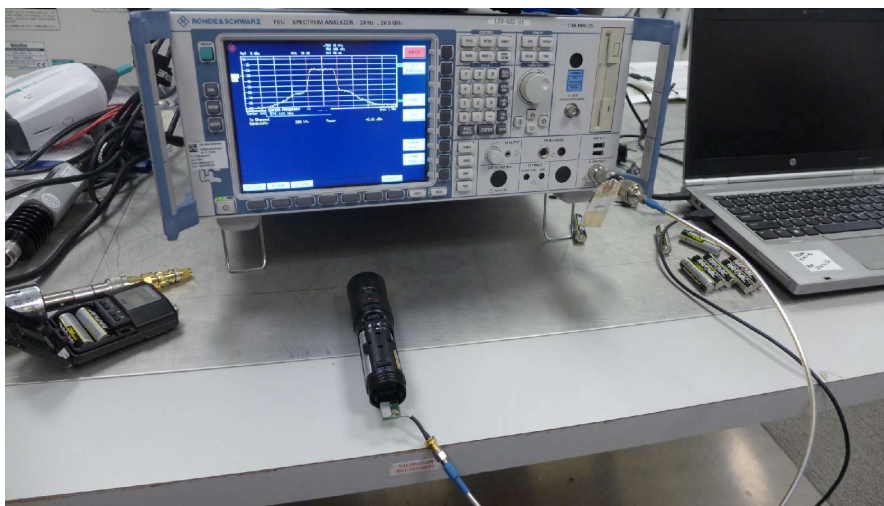
Figure 1: Test setup for Power Output
