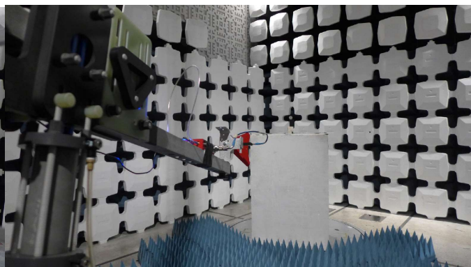
Figure 2: ULXD2 Transmitter Test Setup
