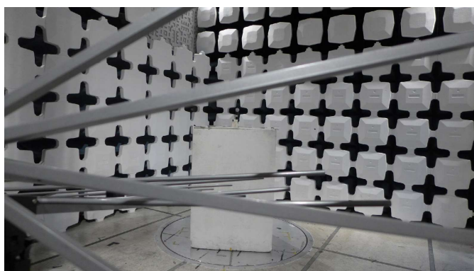
Figure 1: ULXD2 Transmitter Test Setup
