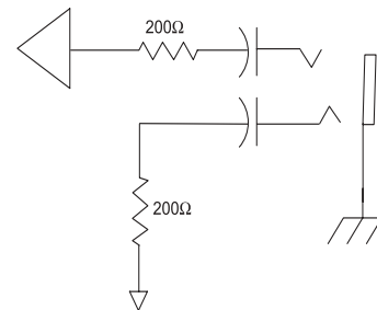
1/4" Phone
