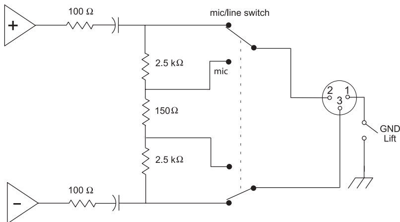
XLR
