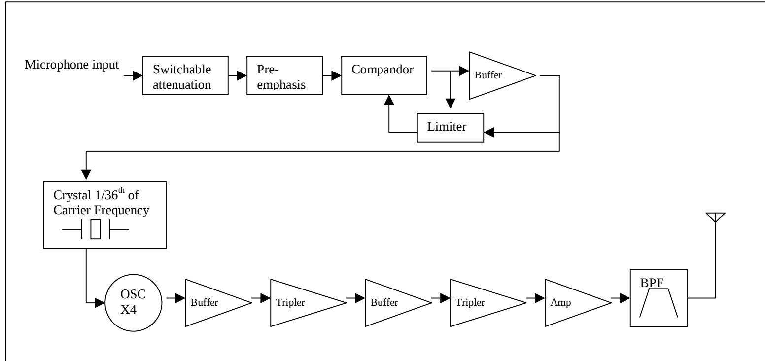
UT2C Block Diagram
