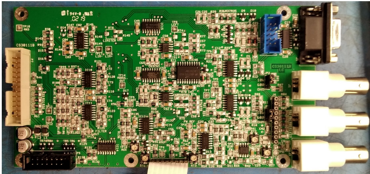
Audio board – top view
