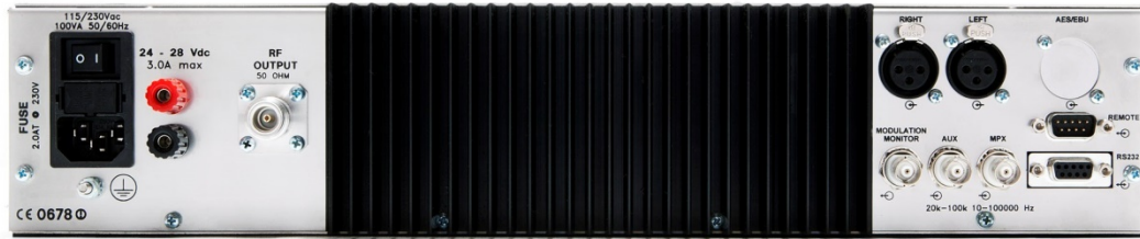
Figure 2 – GTX Transmitter Rear Panel
