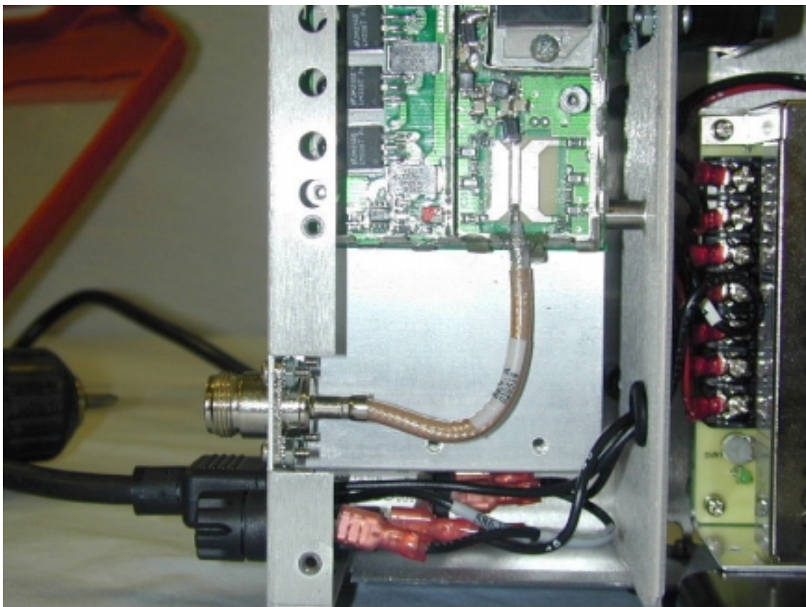
PA board 1
