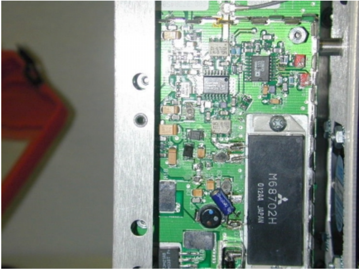
PA Board 3
