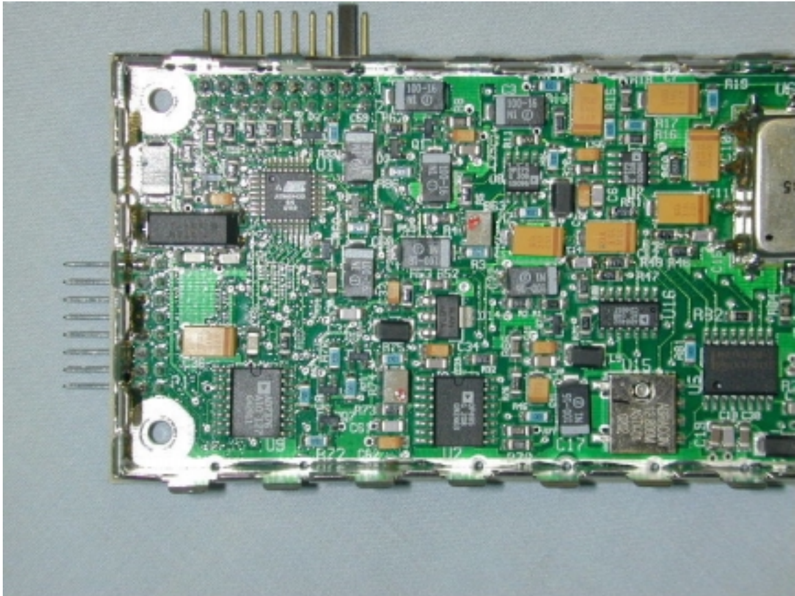
Oscillator Board – Top Closeup 1
