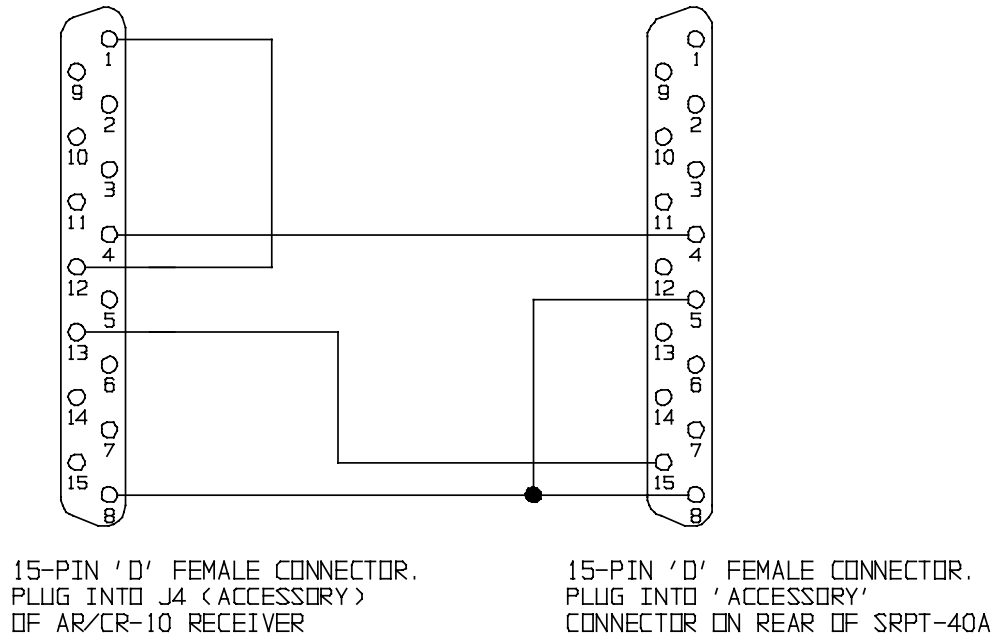
FIG4 - FIXED REPEAT CABLE AR/CR-10 TO SRPT-30/40A MARTI P/N: 585-143
