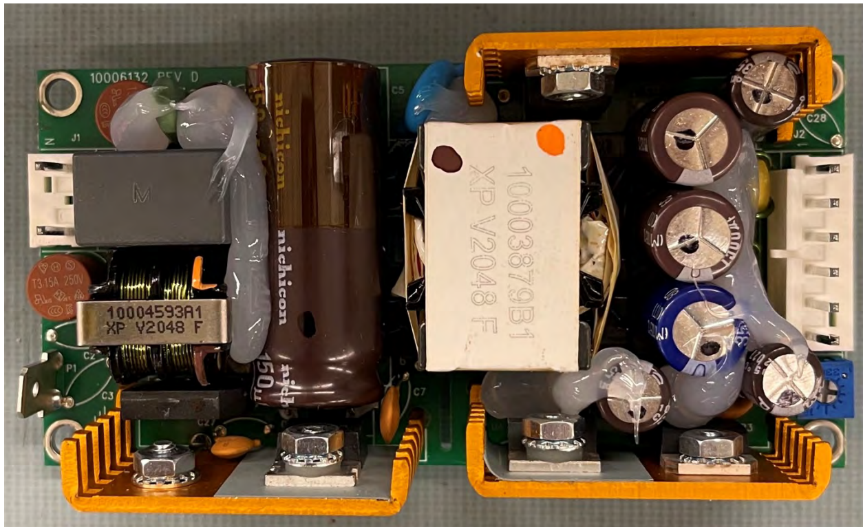
Controller Power Supply – Front View
