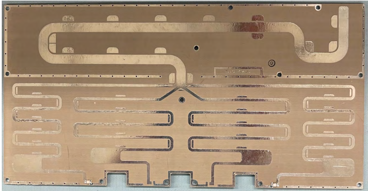
4-Way RF Power Combiner – Front View
