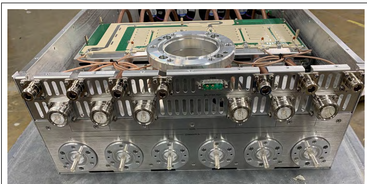
Combiner Rear
