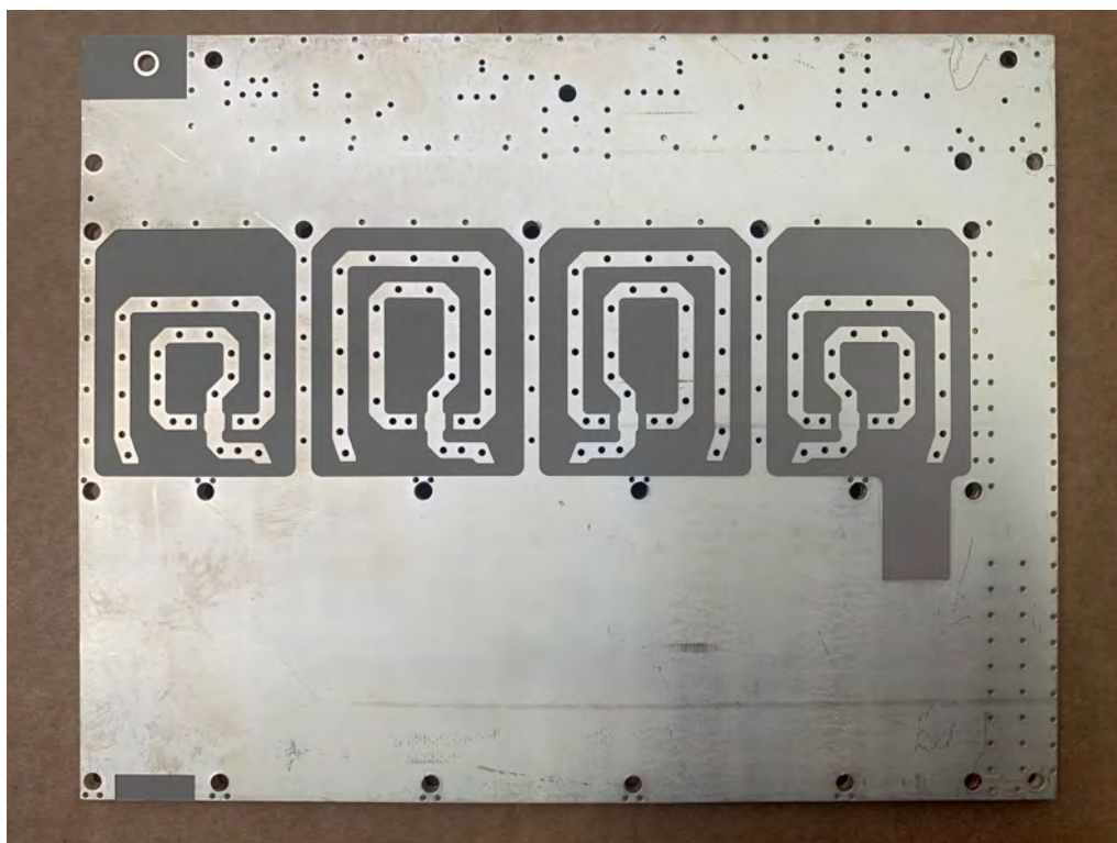
XNK HA455-0 LOW PASS FILTER BOTTOM
