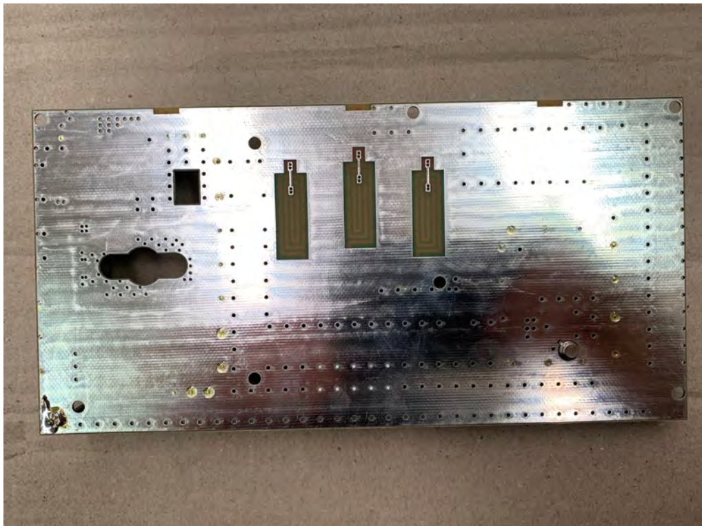
2U3KWA285-1 SPLITTER BOARD 2-WAY 1-1.5KW BOTTOM
