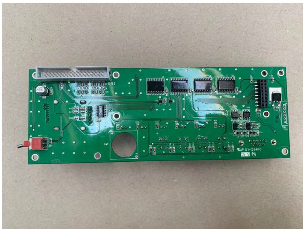
TG2U3A899-3 FRONT PANEL BOARD TOP BOTTOM
