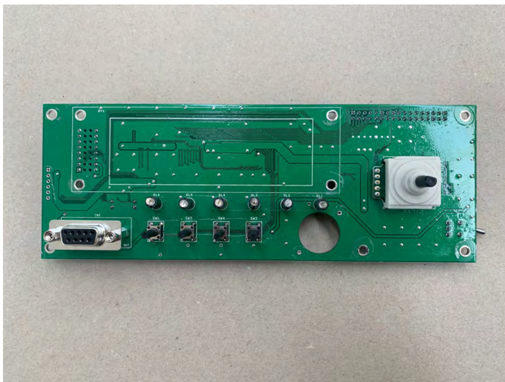
TG2U3A899-3 FRONT PANEL BOARD TOP
