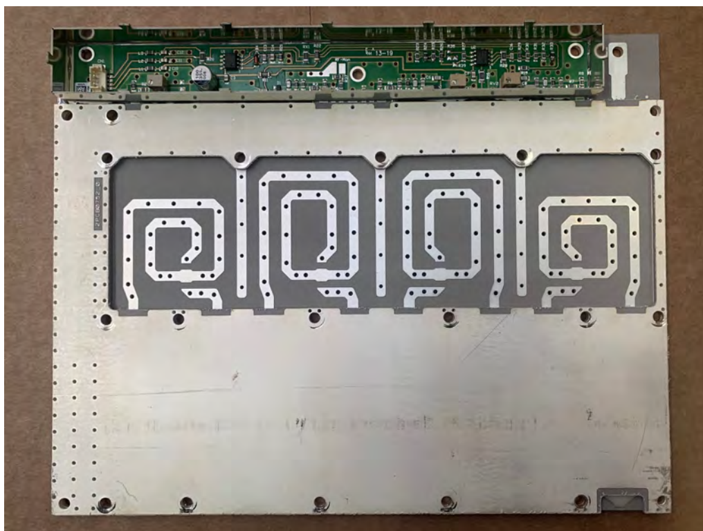
XNK HA455-0 LOW PASS FILTER TOP
