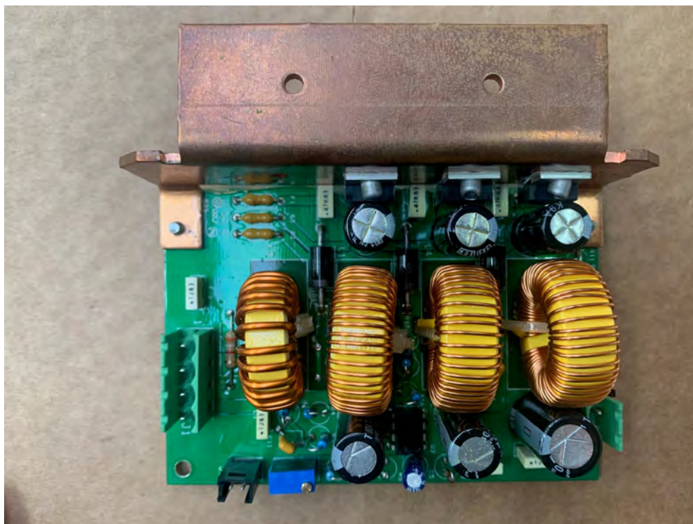
TG2UTA891-5 FAN POWER SUPPLY 3 SECTIONS TOP
