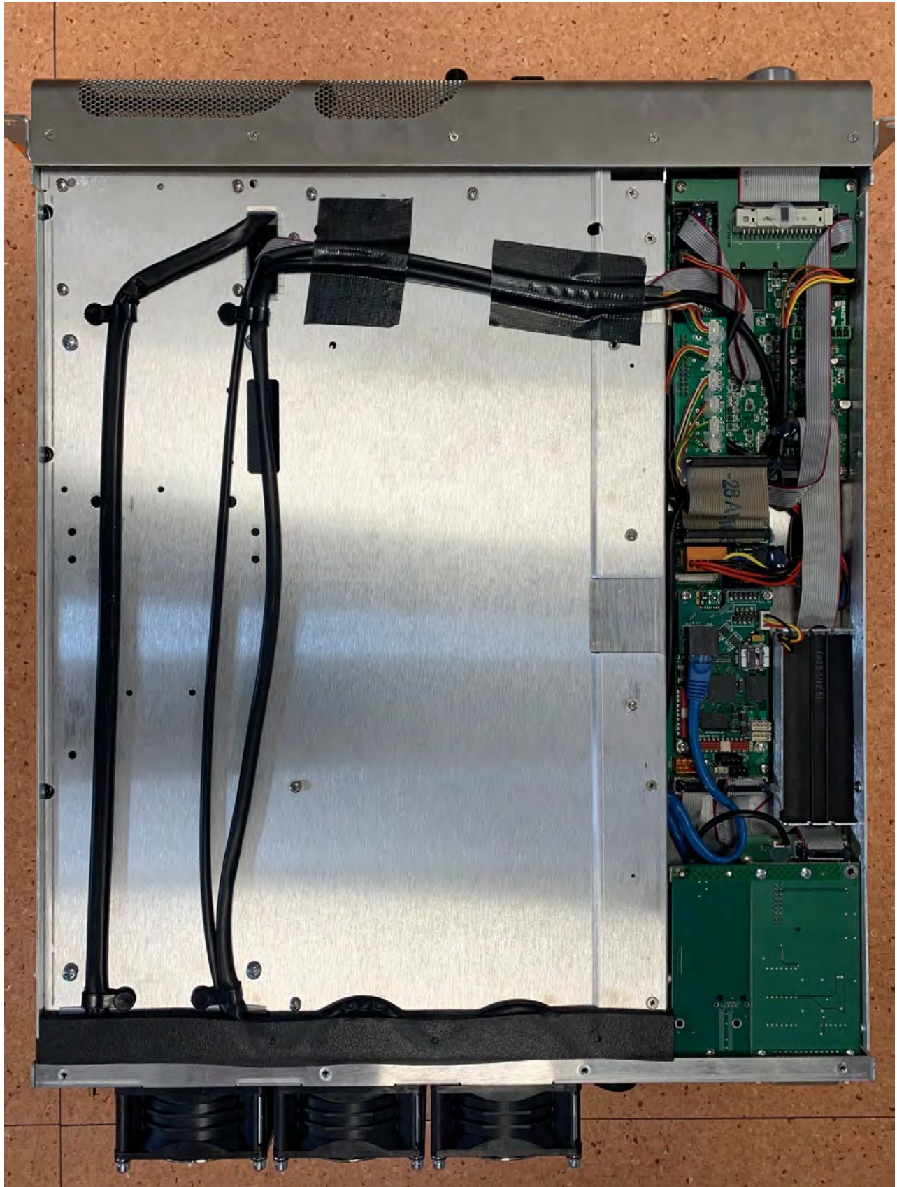
ETG2000 BOTTOM VIEW
