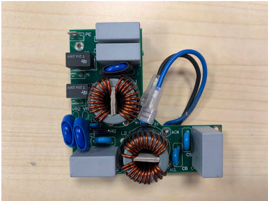
EPSU6A519-1 NETWORK FILTER BOARD TOP
