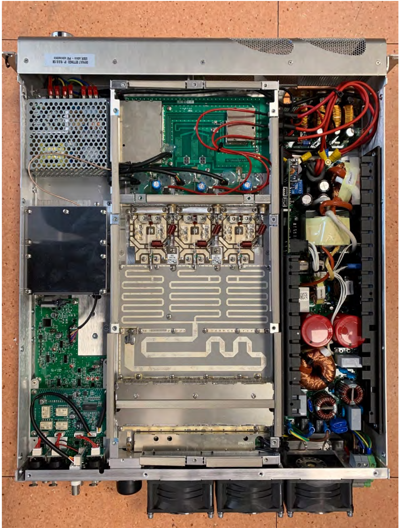
ETG2000 TOP VIEW
