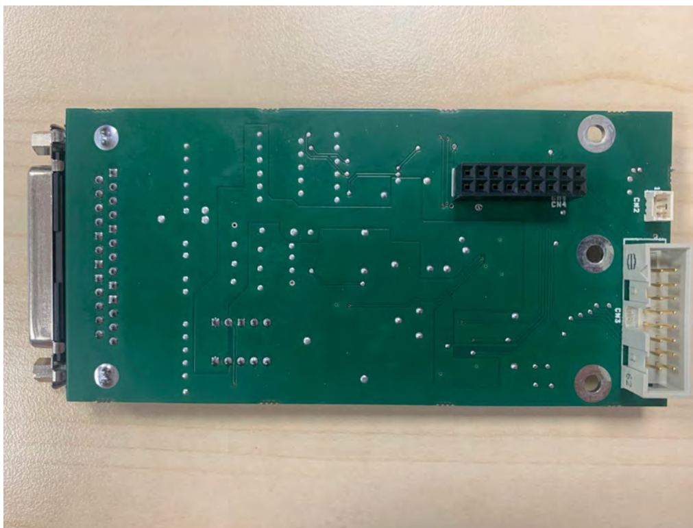
SYS 6A994-2TC/TS BOARD BOTTOM
