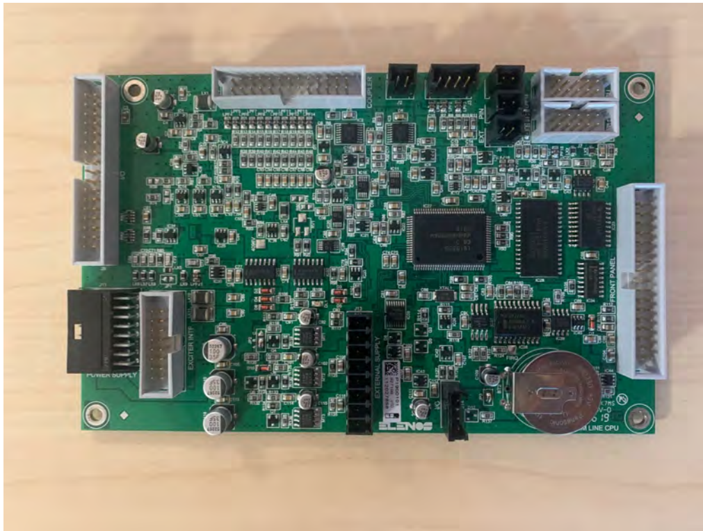
XNK EA453-0 CPU TOP
