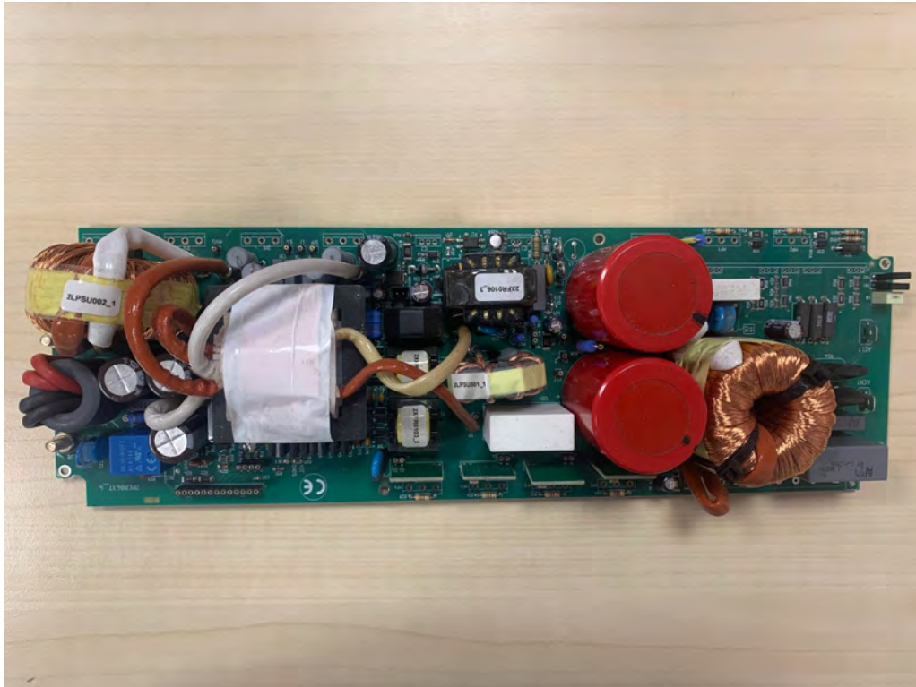
EPSU0A516-5 S3KW PFC POWER BOARD TOP
