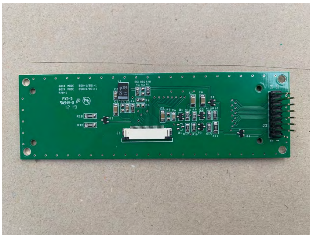
XNK BA452-0 OLED ADAPTER TOP
