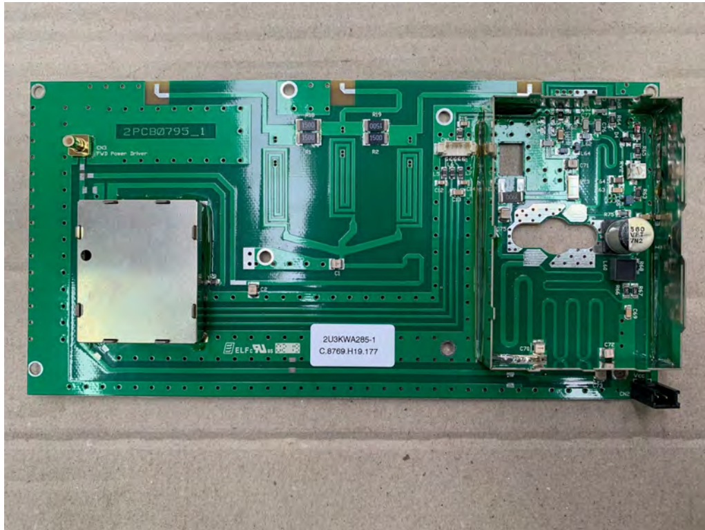
2U3KWA285-1 SPLITTER BOARD 2-WAY 1-1.5KW TOP
