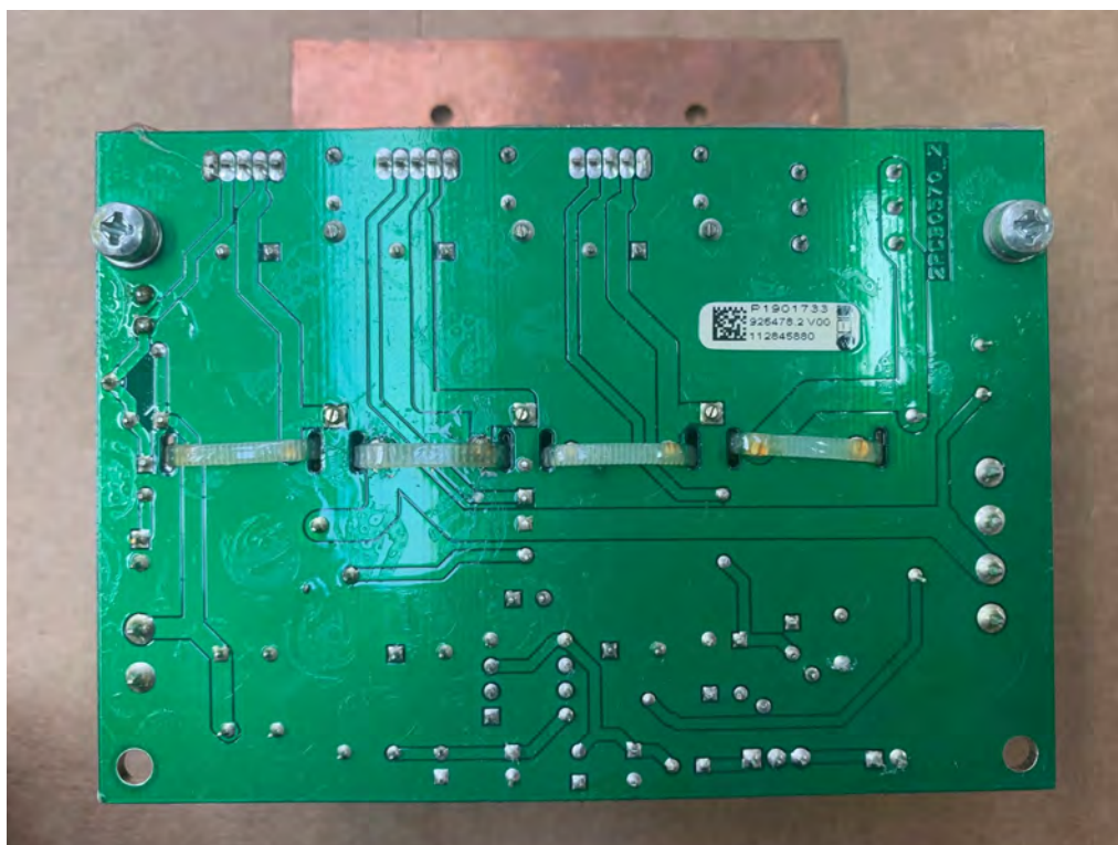
TG2UTA891-5 FAN POWER SUPPLY 3 SECTIONS BOTTOM
