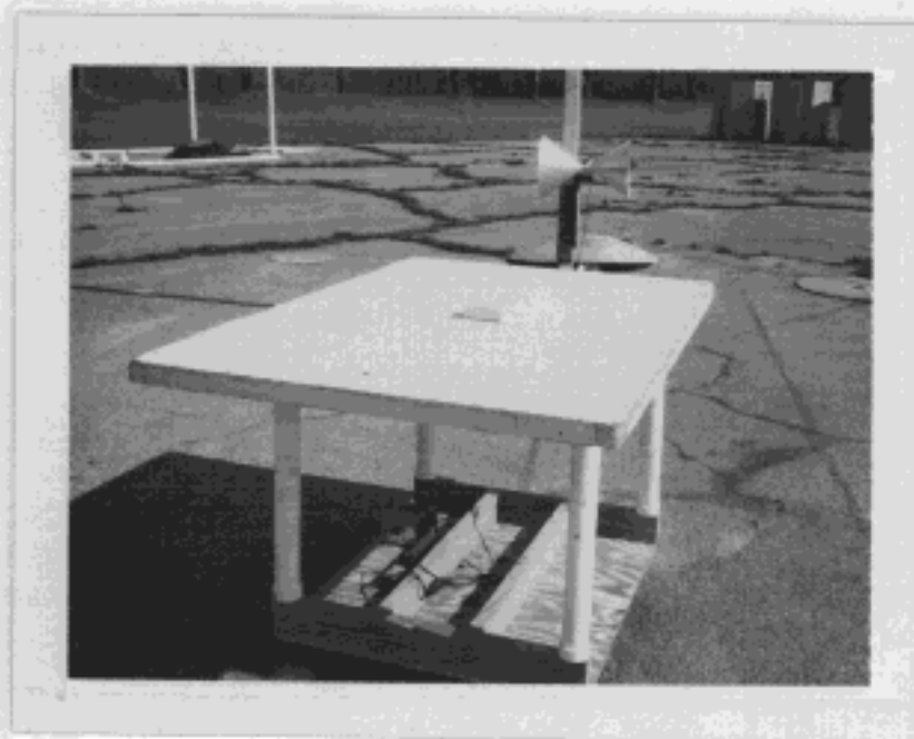
Figure 5.4. DUT on the open-site test table showing the overall view the site.
