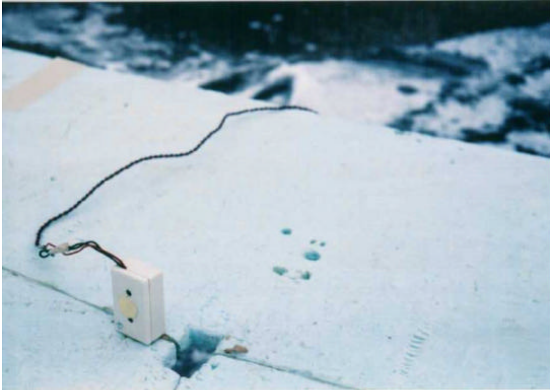
DE47DC3500T Transmitter Close-up on OATS
