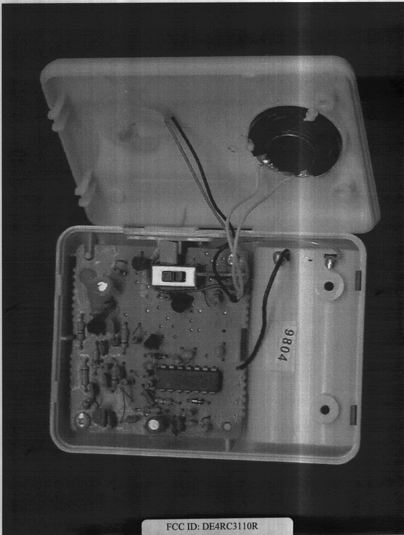
Figure 6.3 Top View, Cover Opened page 18
