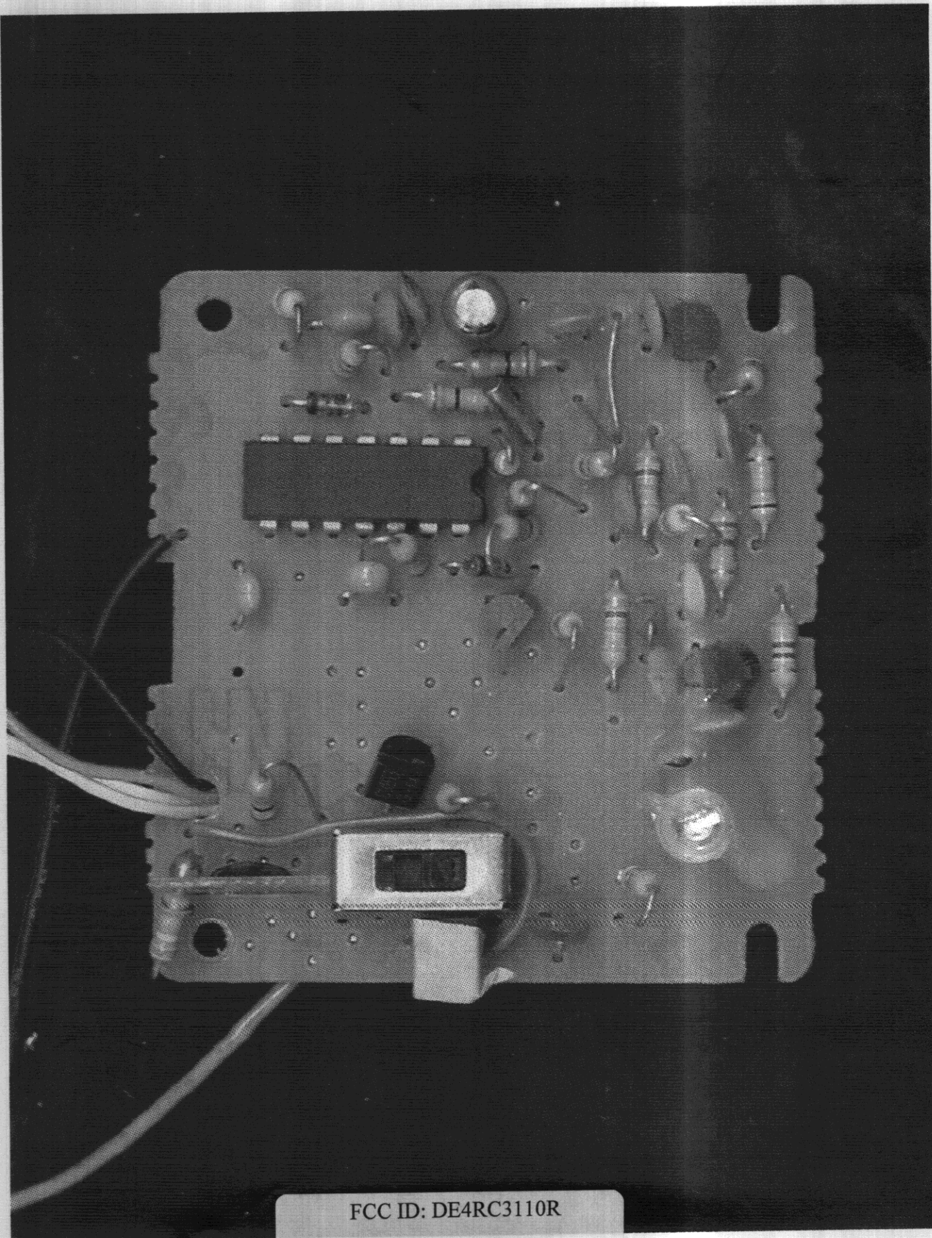
Figure 6.4 PC Board, Component Side page 19
