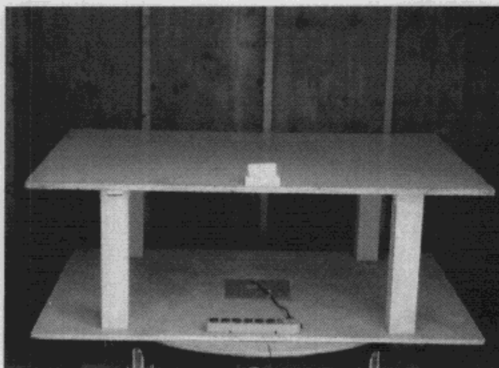
Figure 3.2 Radiated Test Setup, Position 2
