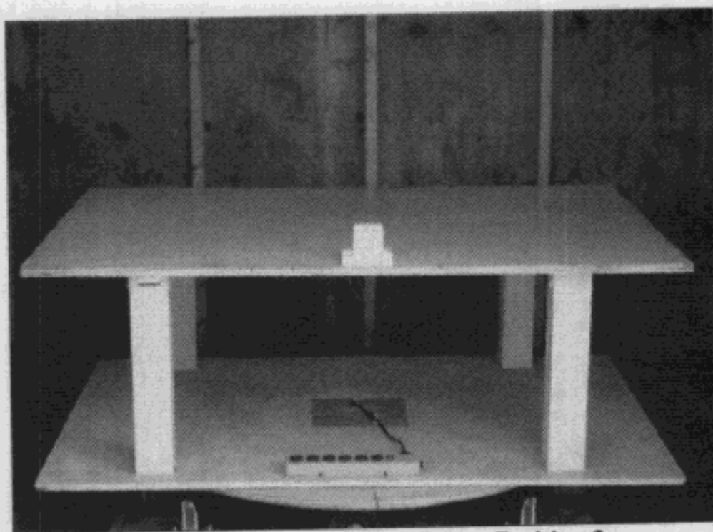
Figure 3.3 Radiated Test Setup, Position 3
