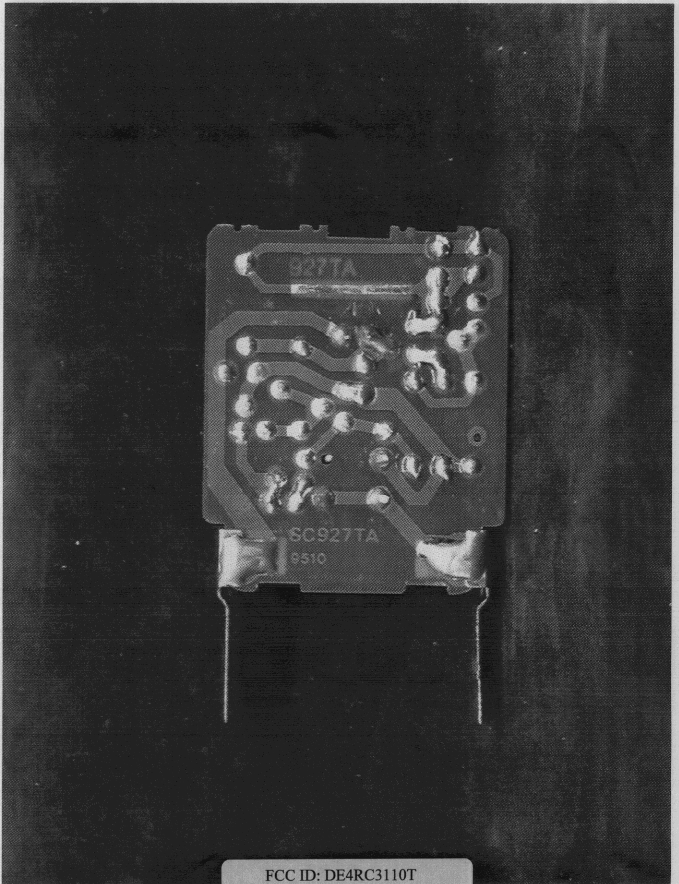
Figure 6.5 PC Board, Foil Side
