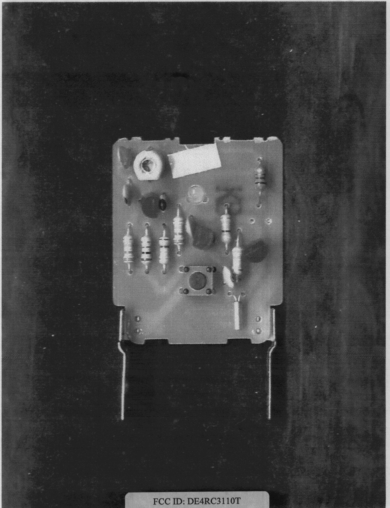
Figure 6.4 PC Board, Component Side page 20
