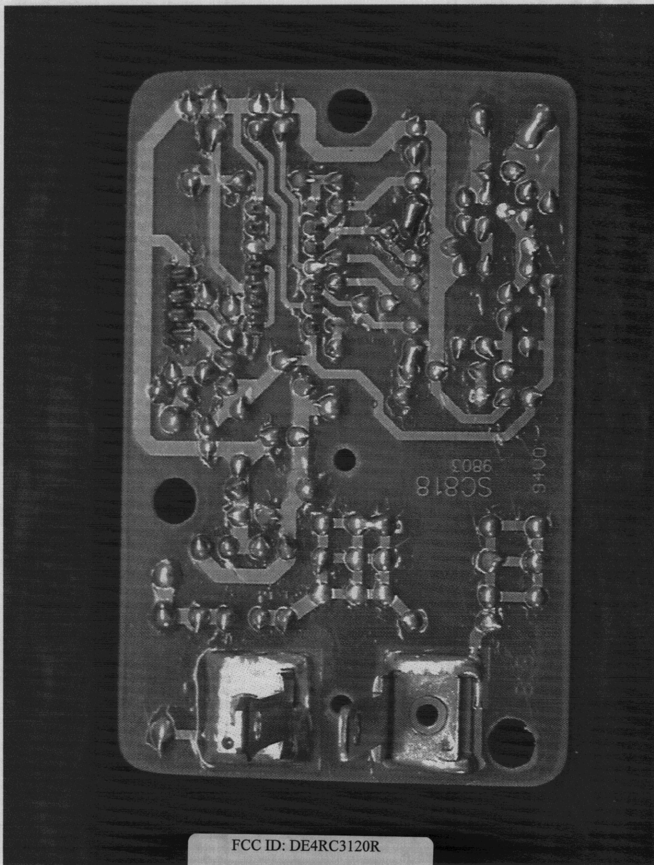
Figure 6.5 PC Board, Foil Side page 24
