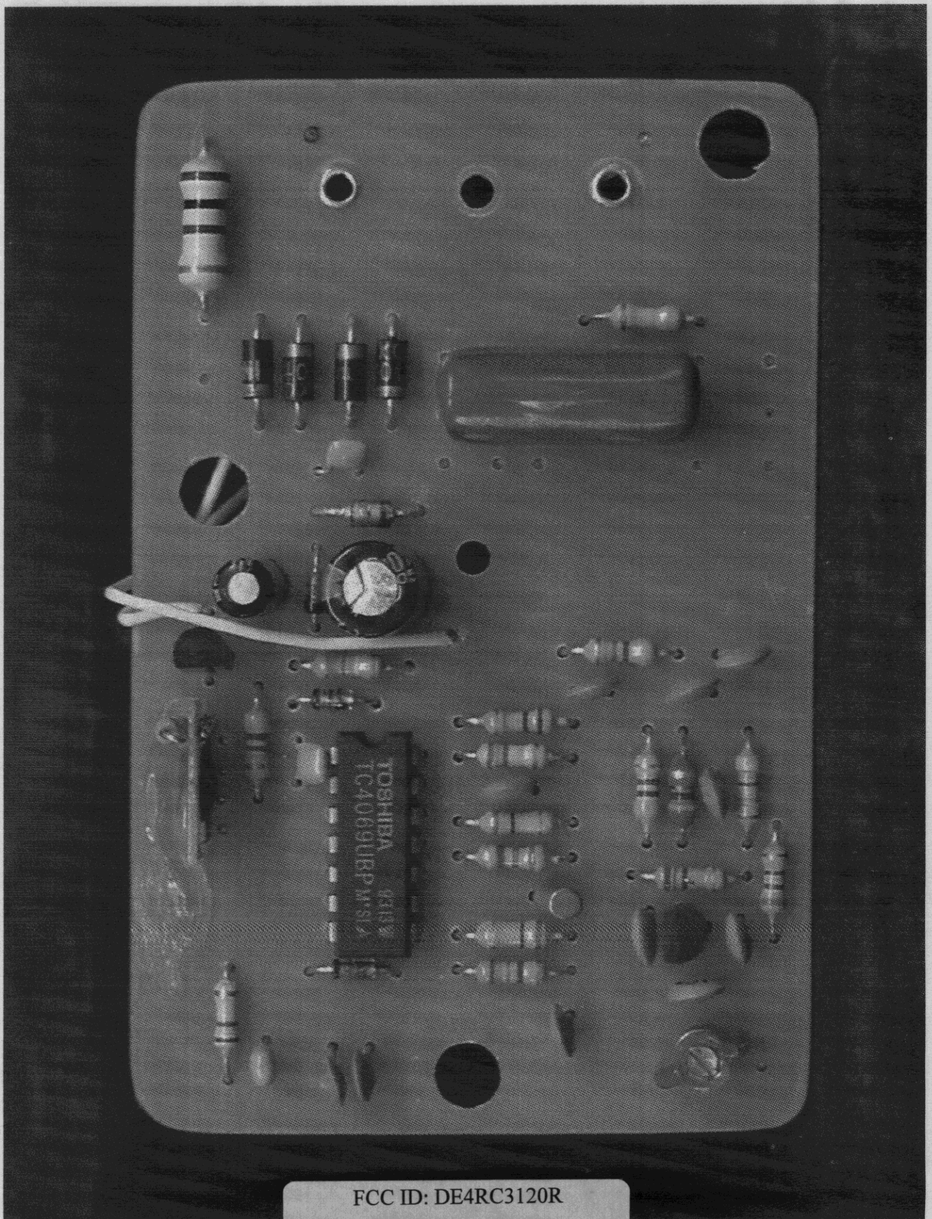
Figure 6.4 PC Board, Component Side page 23
