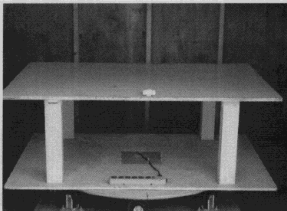
Figure 3.1 Radiated Test Setup, Position 1
