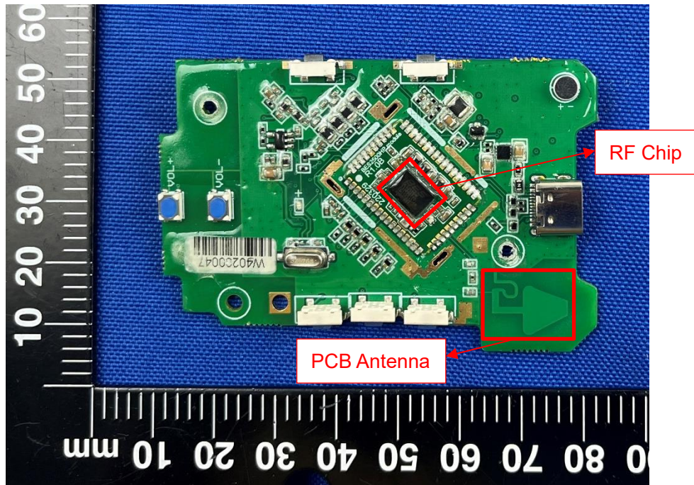
MAIN BOARD REAR VIEW (WITHOUT SHIELDING)
