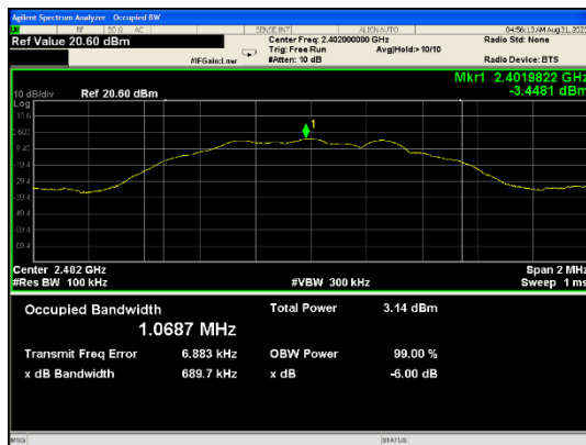
FCC OBW – Low Channel
