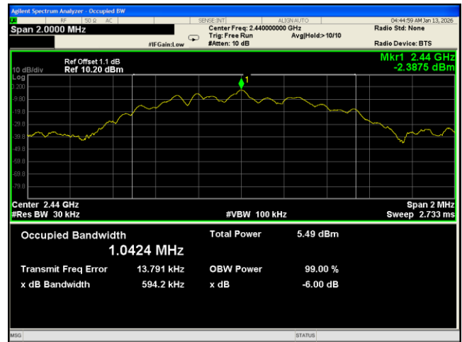
RSS-Gen FCC OBW – Mid Channel
