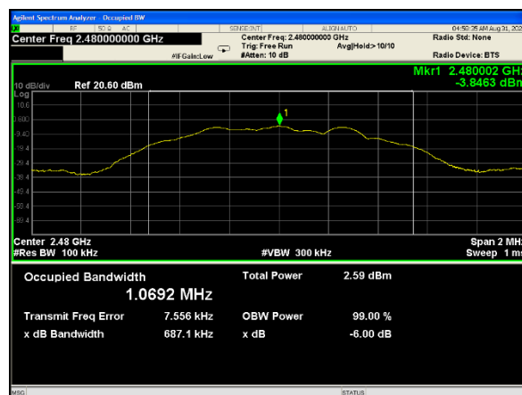
FCC OBW – High Channel
