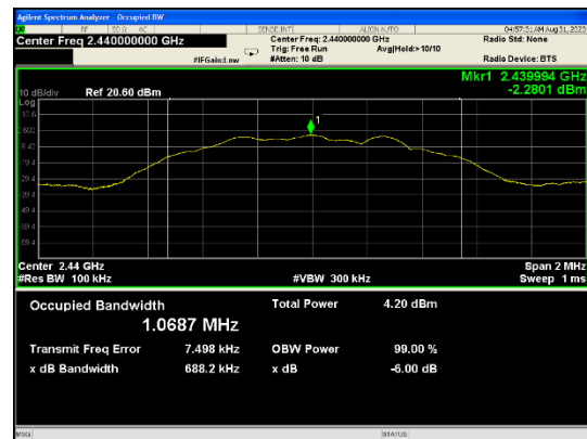
FCC OBW – Mid Channel
