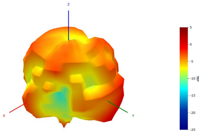
Measured Antenna Gain 2025-11-14 3M Personal Safety XDBFE Port-1, Tab: Magnitude
