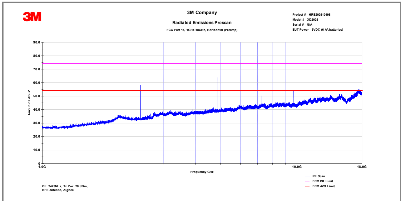
FCC Part 15.209 Radiated Emissions in restricted band - BFE Antenna
