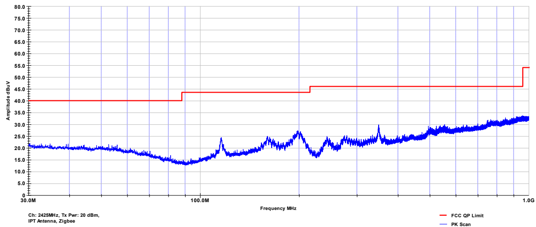
FCC Part 15.209 Radiated Emissions in restricted band - IPT Antenna
