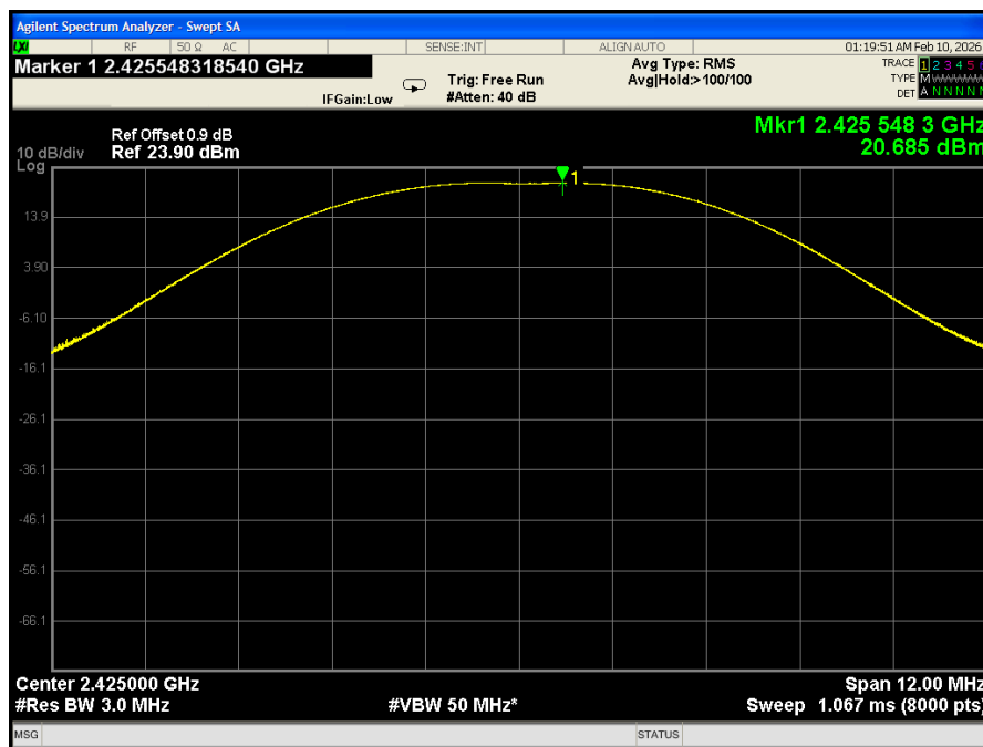
Conducted RF Power
