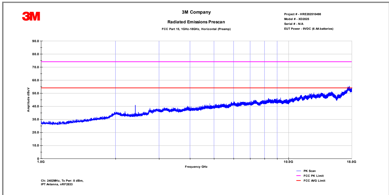
FCC Part 15.209 Radiated Emissions in restricted band - IPT Antenna, Low Ch.
