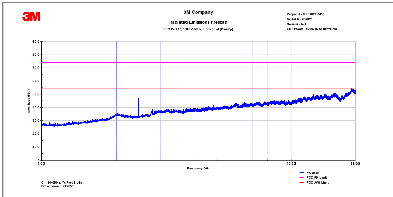
FCC Part 15.209 Radiated Emissions in restricted band - IPT Antenna, Mid Ch.
