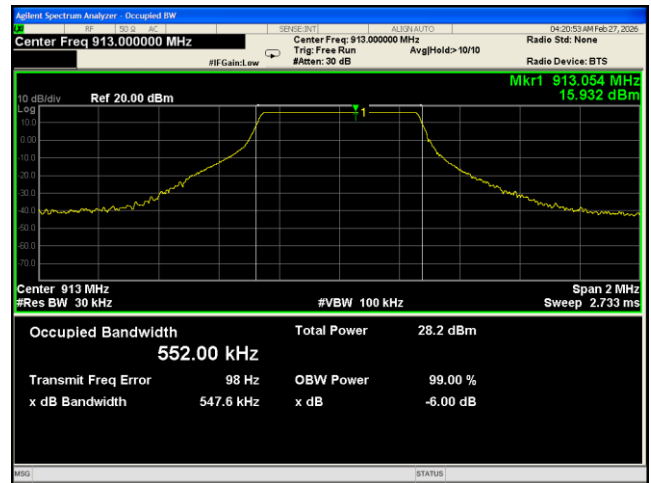
RSS Gen – Mid Channel
