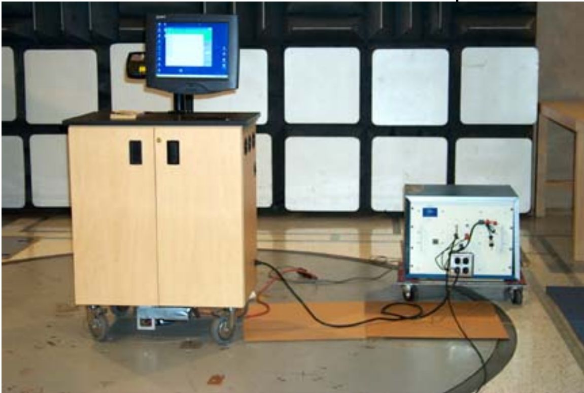
Emissions Bandwidth and Spurious Emissions below 30 MHz Test Setup
