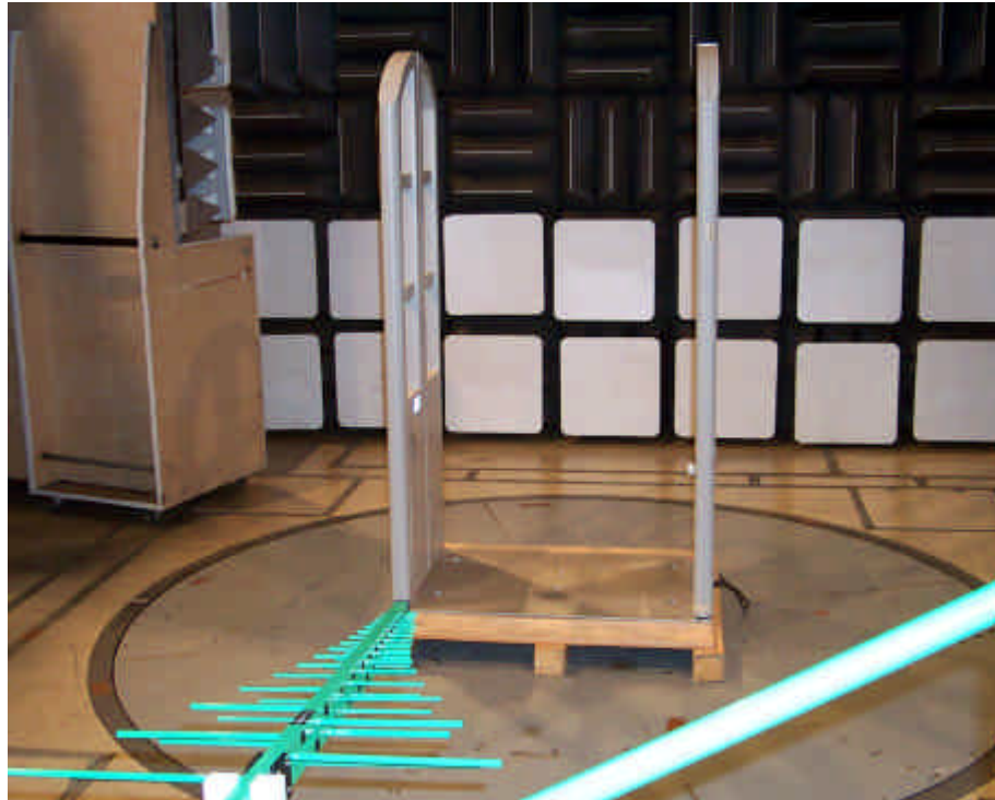
Radiated Emissions (30-1000 MHz)
