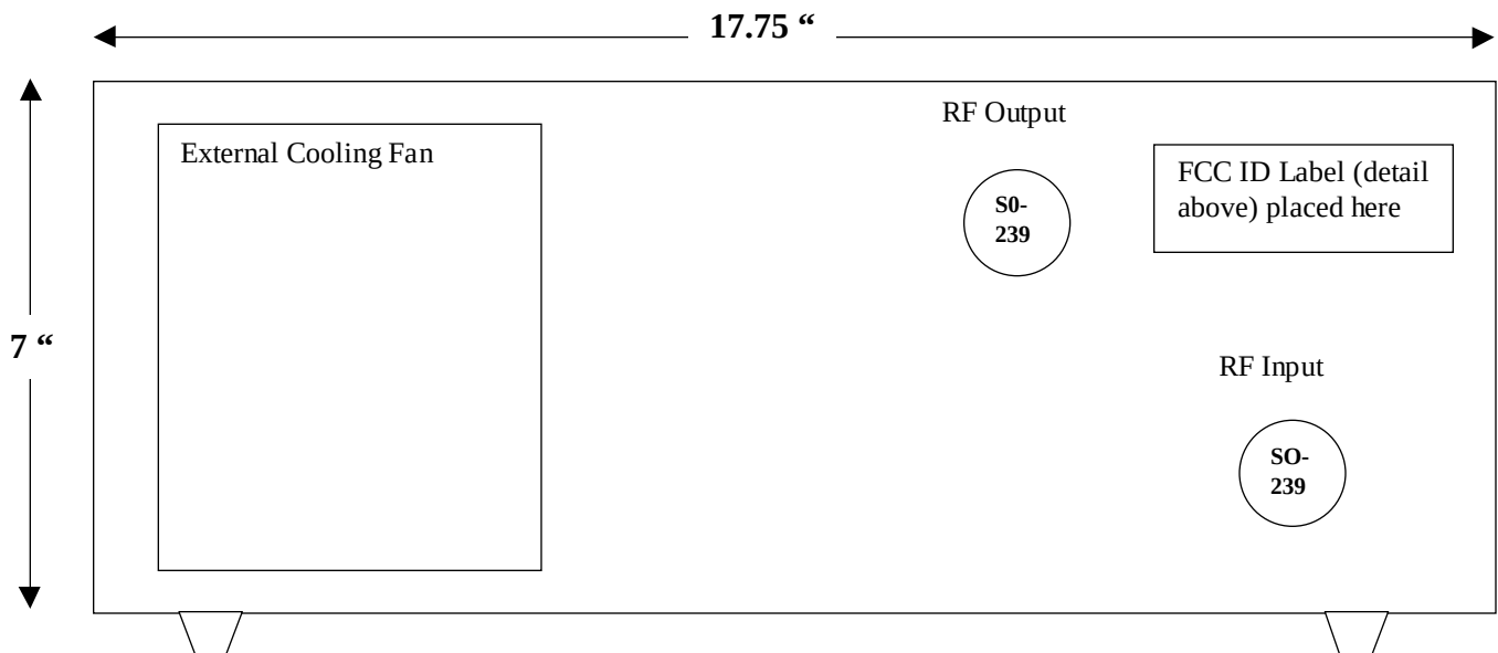
Figure 2. Alpha 6 Rear Panel Detail Showing Placement of FCC Label
