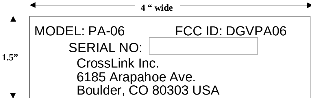
Figure 1. Details of Alpha 6 FCC ID Equipment Label
