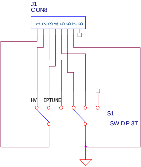
MULTIMETER SWITCH
