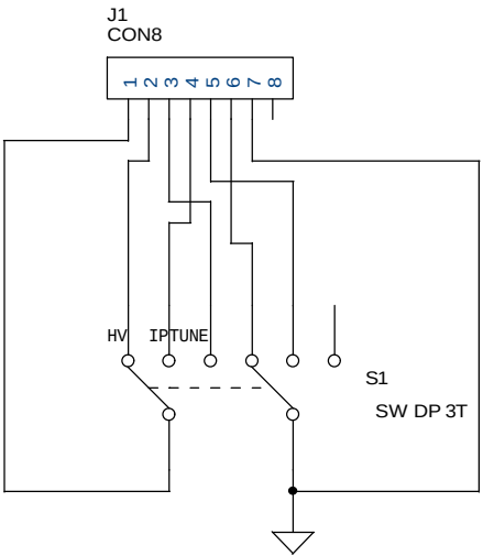
MULTIMETER SWITCH
