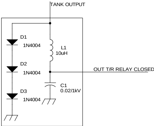
T/R STATUS BOARD ABX-X407
