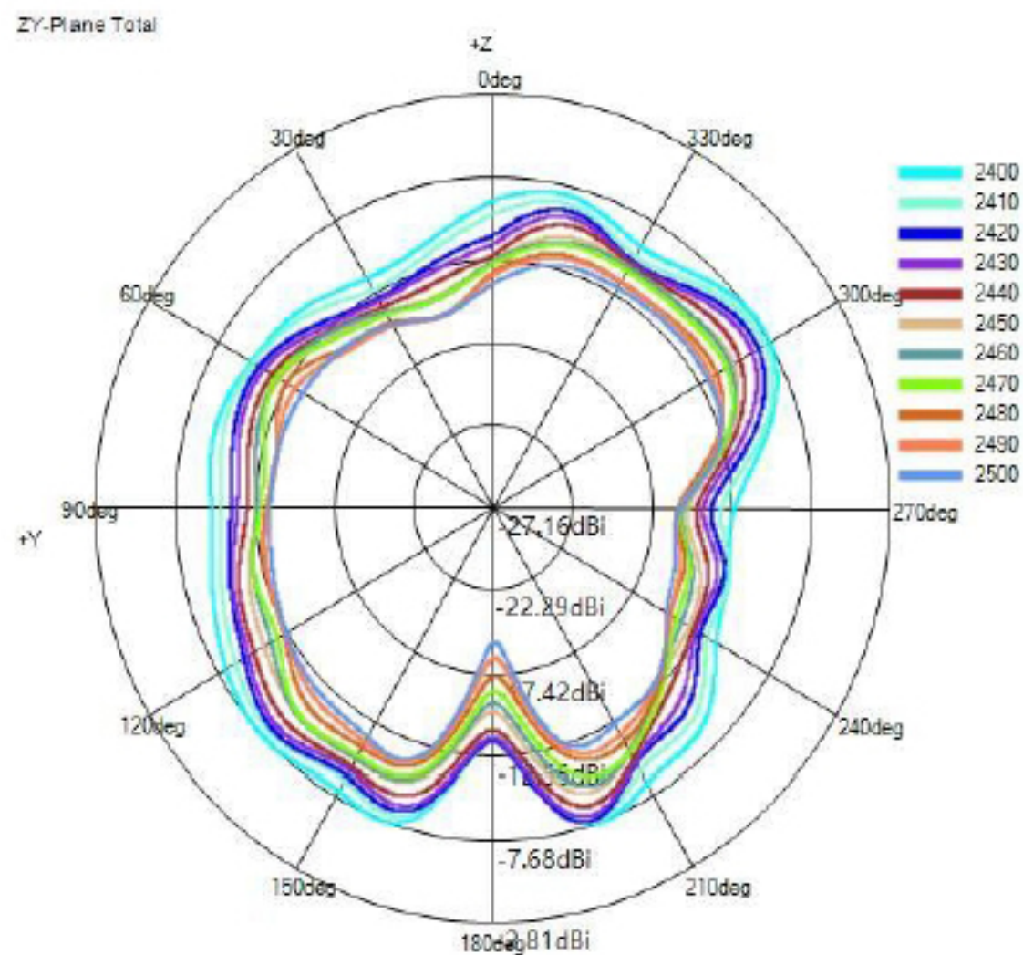
(2) Y-Z Plane(unit:dBi):
