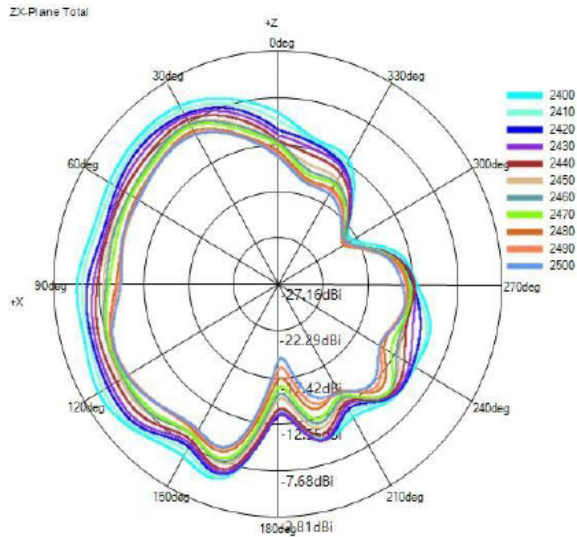
(1) X-Z Plane(unit:dBi):
