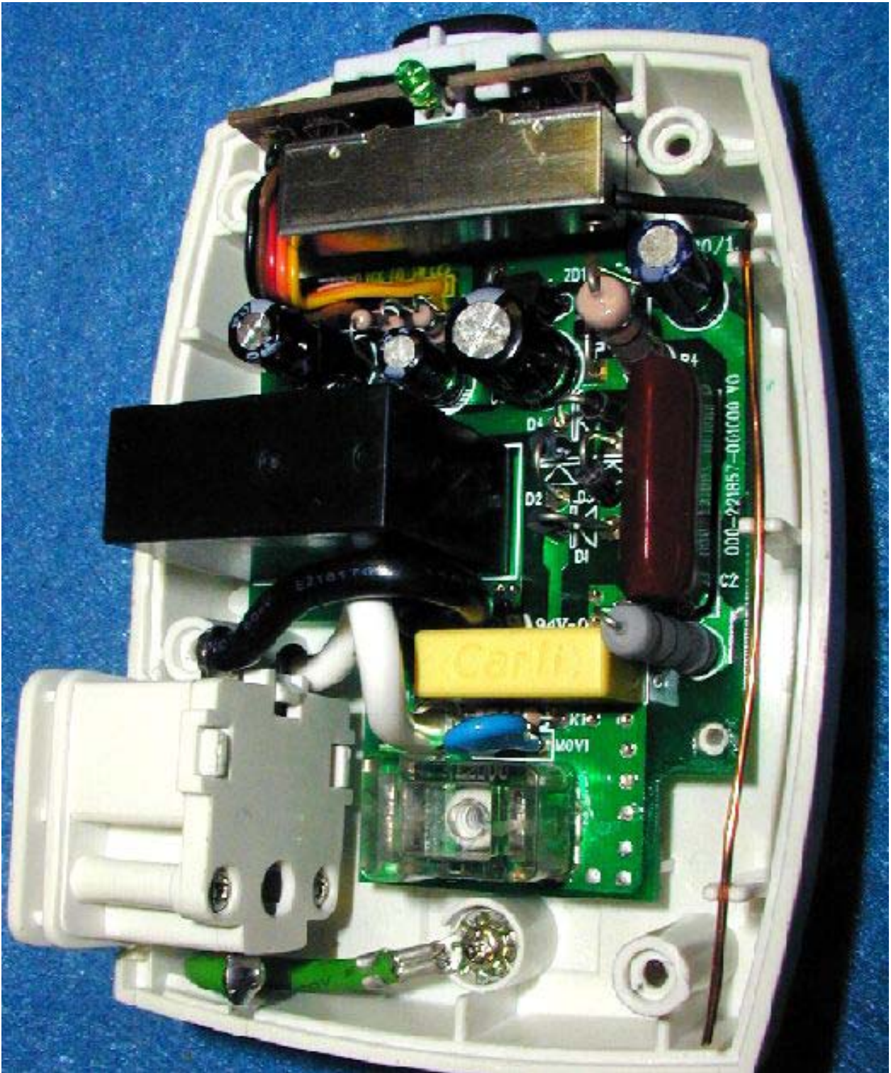
TOP VIEW OF MOTHERBOARD
